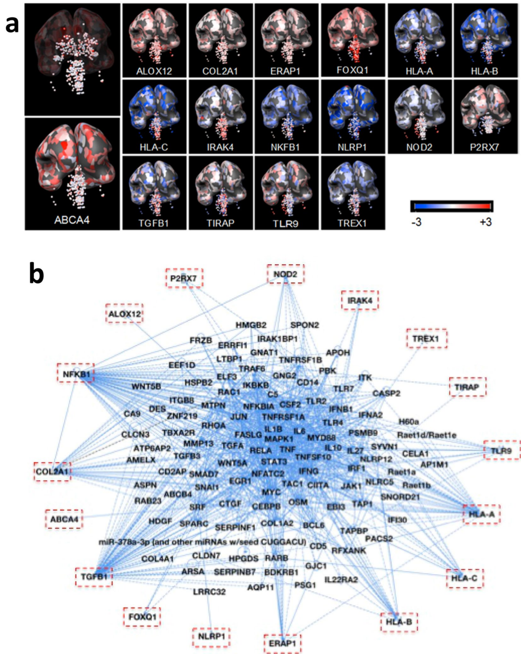
Figure 2. Susceptibility genetics. (a) Expression and localization in human brain utilizing Allen Brain Atlas of genes with alleles conferring susceptibility to congenital toxoplasmosis in National Collaborative Chicago Based Congenital Toxoplasmosis Study (NCCCTS). Transcript expression is visualized for brain of the youngest donor (H0351.2001, 24 years, male, African-American). Z-score of microarray data ranges between -3 and +3 to quantify the lowest to highest expression (see Supplement B: Table S2). (b) Ingenuity Pathway Analysis (IPA) of NCCCTS susceptibility genes and upstream regulators. Cut off of p value at 5 \times 10^{-3} generated a network of 117 predicted upstream regulators (see Supplement B: Table 2). Upstream regulators and susceptibility genes are consolidated/bundled and graphically mapped. Susceptibility genes are manually relocated in IPA graphic to show connectivity to upstream regulators. Note NF \kappa B and TGF \beta are central nodes that are visual.
